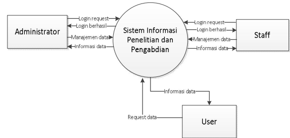
Gbr. 4 DCD (Data Context Diagram)
