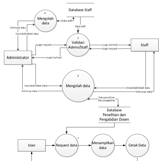
Gbr. 5 DFD (Data Flow Diagram)
