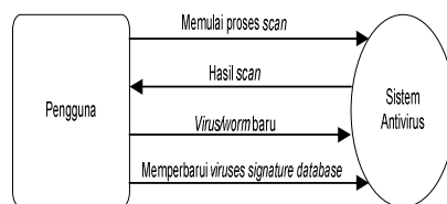
Gambar 6. Context Diagram
